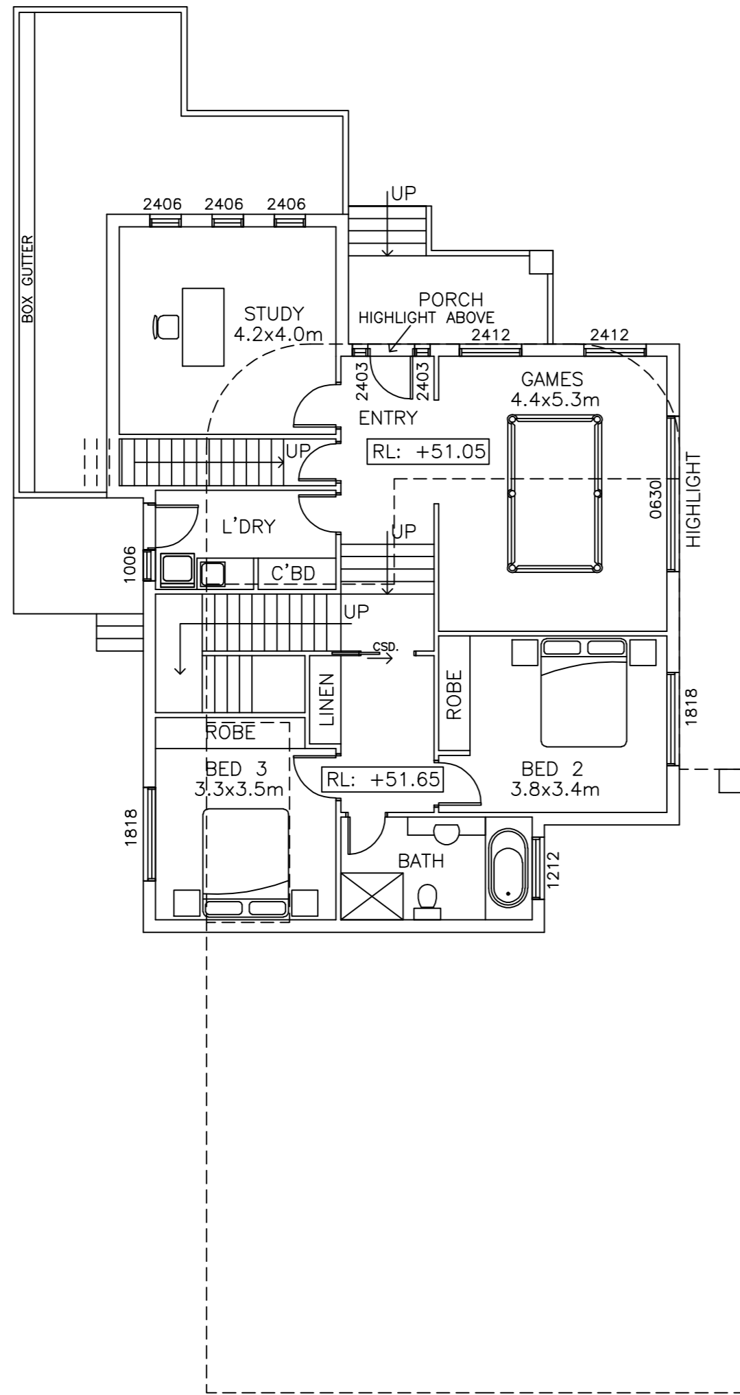
GROUND FLOOR
