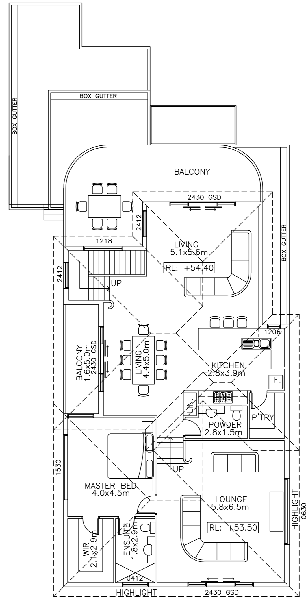
FIRST FLOOR
